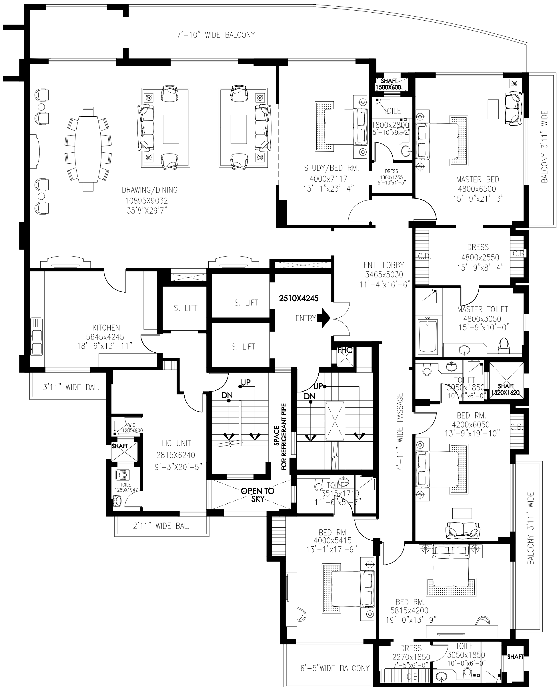
TENTATIVE TYPICAL APARTMENT PLAN (SECOND TO 8TH FLOOR) APARTMENT TYPE B & LIG UNIT
